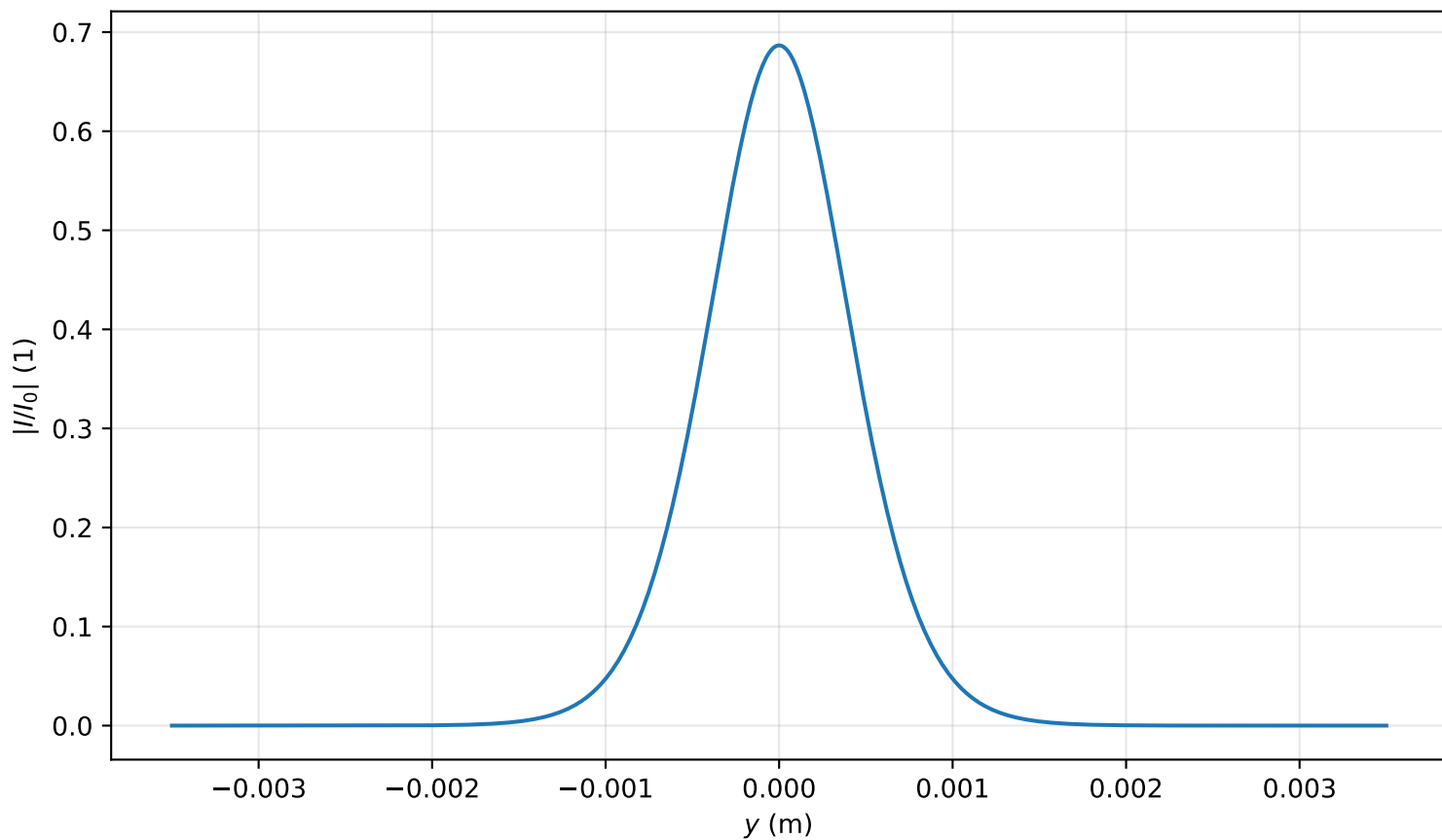
Intensity profile I(x=0, y, z=2.149)/I_0 , P_{in}=0.4P_{cr} , artificial time
